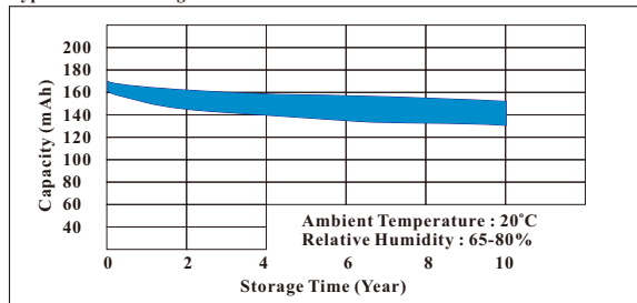
Typical Self Discharge Characteristics
